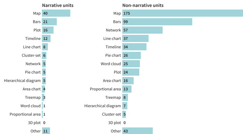
Figure 26 Frequency of visualisation techniques in narrative (left; n = 116) and non-narrative (right; n = 471) visualisation-interaction units.
