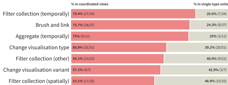
Figure 21 Proportion of allowable actions that occur more often in multi-type coordinated units, split by their frequency in coordinated views versus single-type units.
